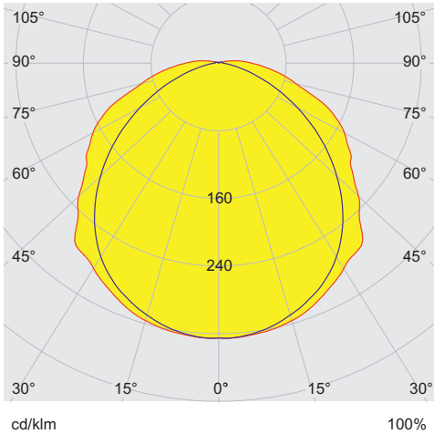
typical with diffuser, clear translucent cover
