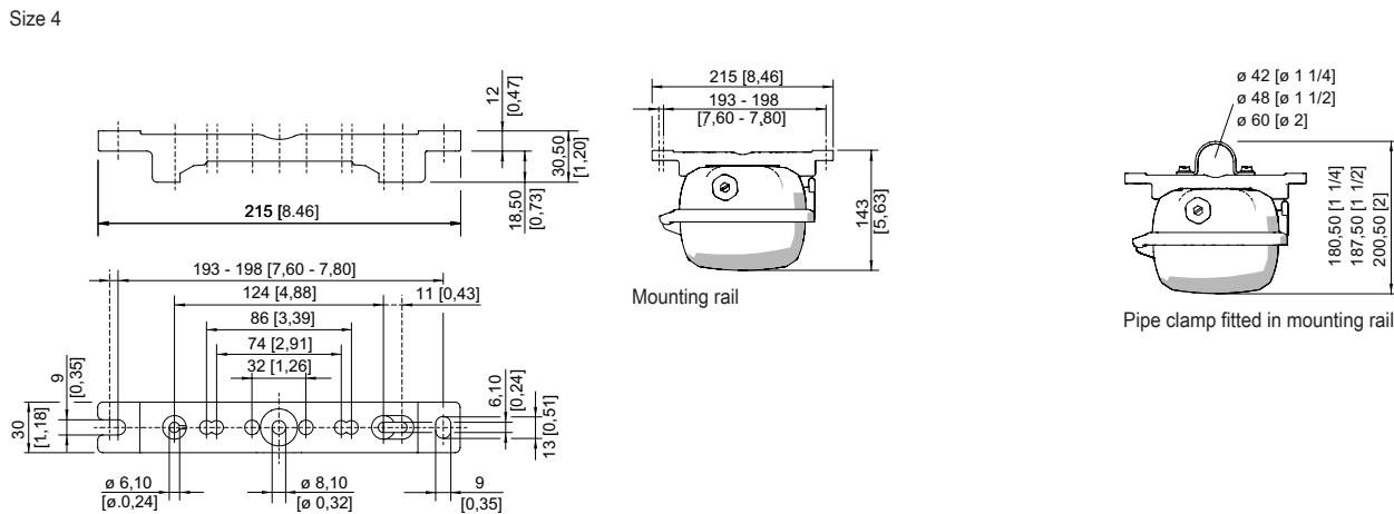
Mounting rail
