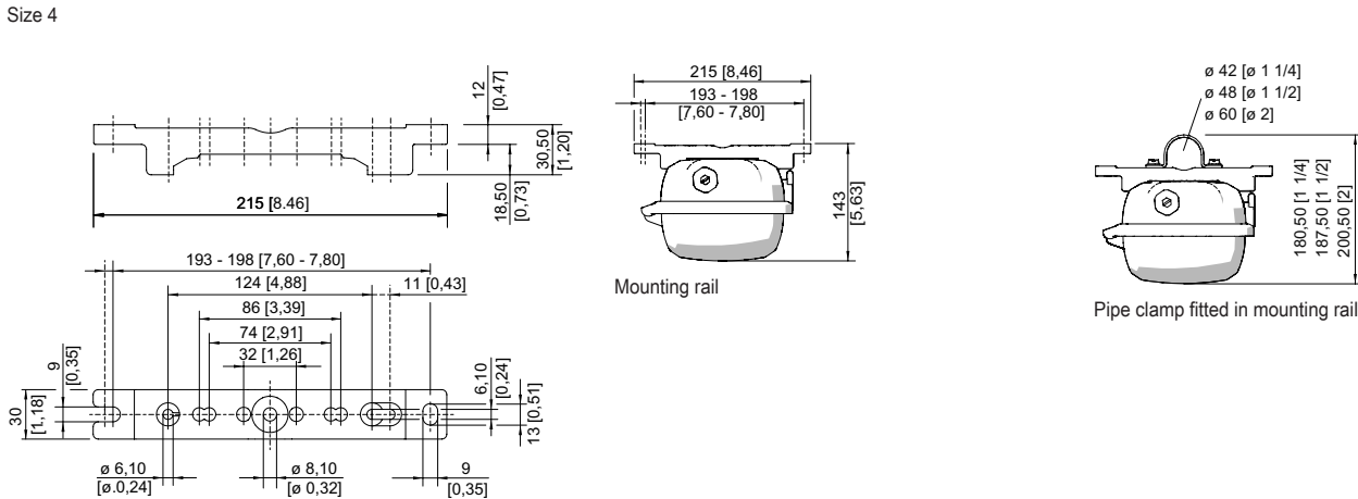
Mounting rail
