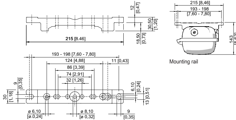
Mounting rail
