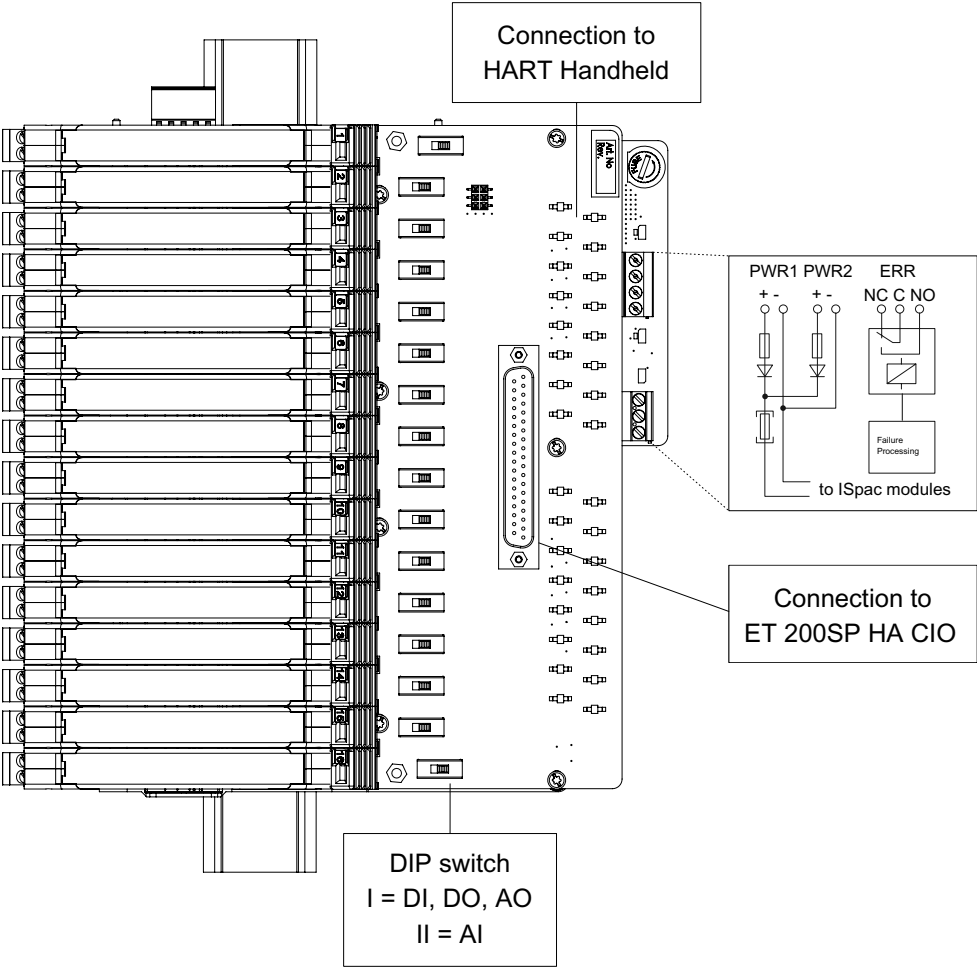
Connection diagram 9295/21AH-SI3-01A5
