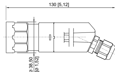
8003/...-001 pushbutton
