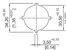
Punch pattern
