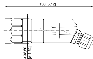
8003/...-727 lockable rotary actuator
