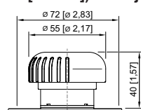
8008/...-015 mushroom stay-put button dia. 55 mm
