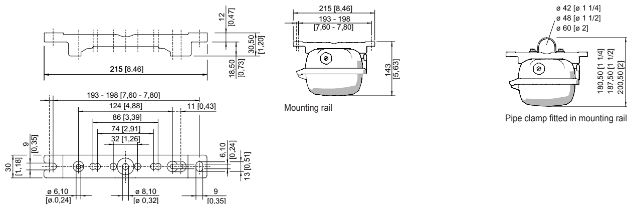
Mounting rail
