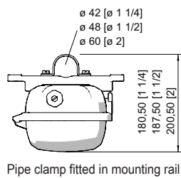
Pipe clamp fitted in mounting rail
