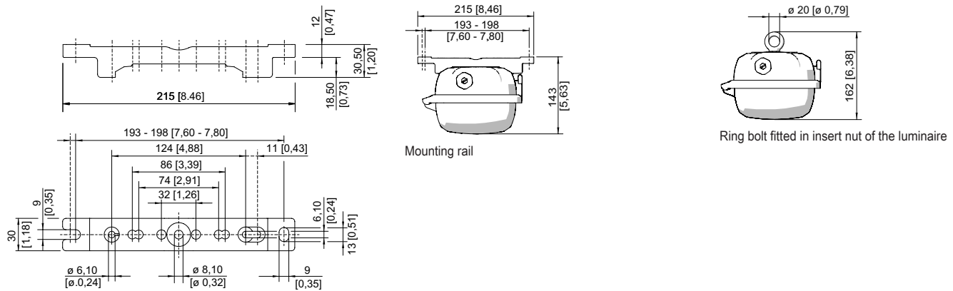
Mounting rail
