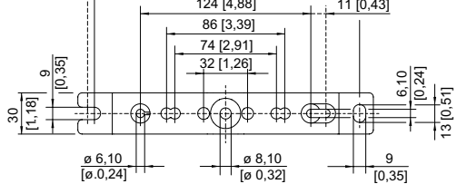
Mounting rail
