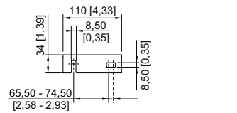
Wall mounting bracket fitted in mounting rail
