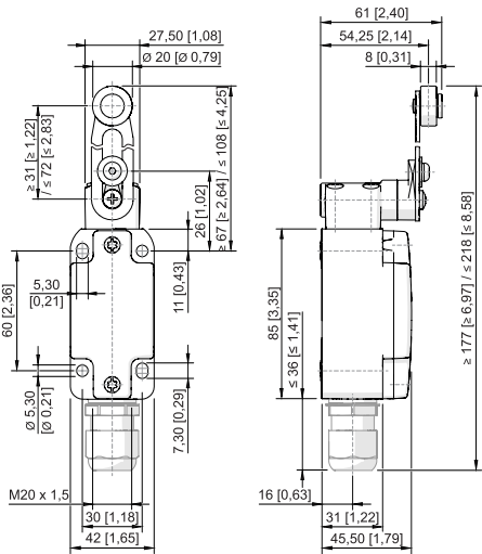
Swivelling lever 8070/2-3-DS-U60
