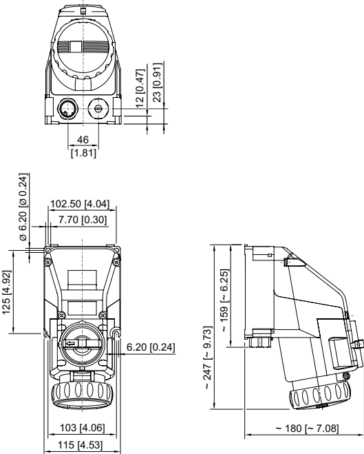
4-pole/5-pole wall-mounting receptacle
