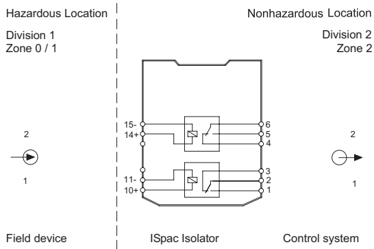
Connection Diagram 9172/20-11-00
