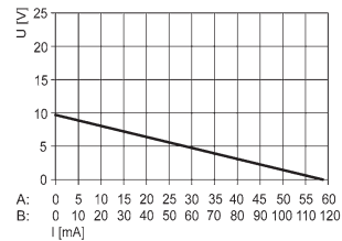
9175/0-12-11, 9176/0-12-00 output characteristic
