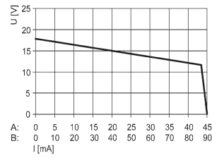
Output characteristic 9175/0-14-11, 9176/0-14-00
