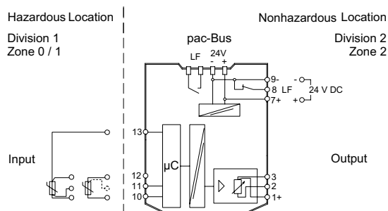
Connection Diagram 9180/10-77-11
