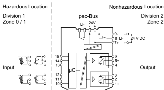
Connection Diagram 9180/20-77-11
