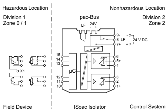
Connection diagram 9180/21-77-11
