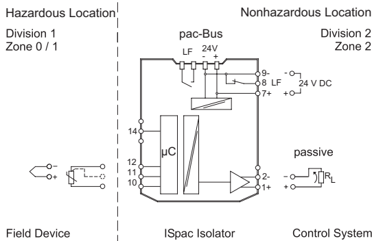
Connection diagram 9182/10-51-11; 9182/10-51-13
