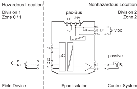
Connection diagram 9182/10-51-11; 9182/10-51-13
