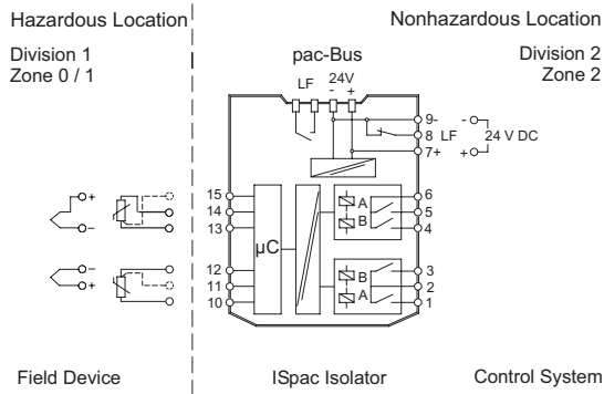
Connection diagram 9182/20-50-12
