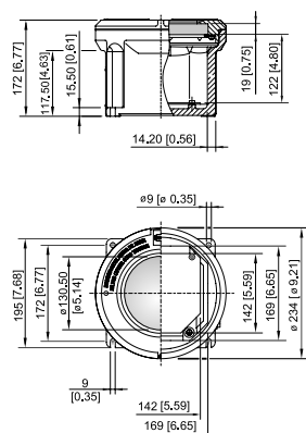
Enclosure size 3 with inspection window
