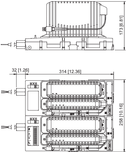
Ethernet CPU Module & Power Module with redundant Socket for Div. 1
