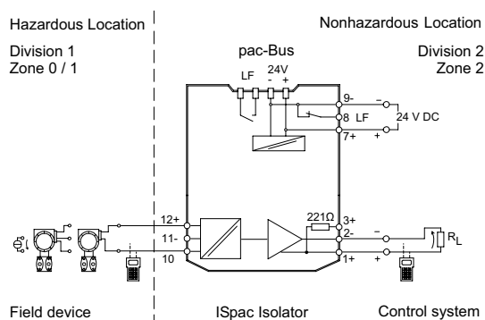
Connection diagram 9160/13-11-13
