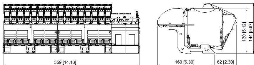
9419/08R bus-Carrier for 16 fieldbus segments
