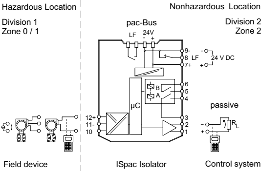
Connection diagram 9162/13-11-14
