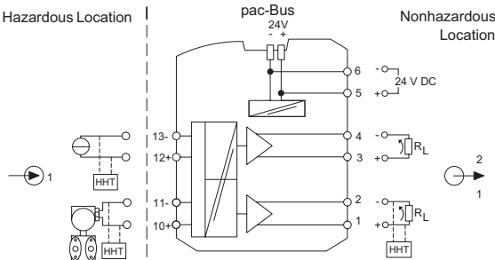
Connection diagram 9260/19-11-10
