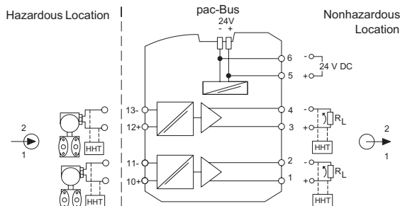
Connection diagram 9260/23-11-10
