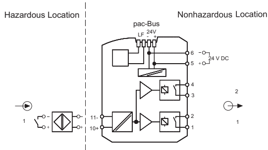
Connection diagram 9270/11-17-15
