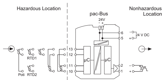
Connection diagram 9282/11-51-16
