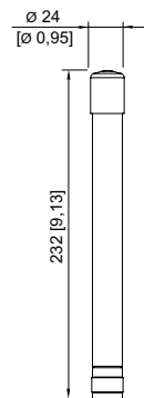
Antenne type 9790/1-2458-NTM-53
