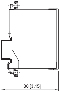
Installation sur support rail DIN NS 35/15
