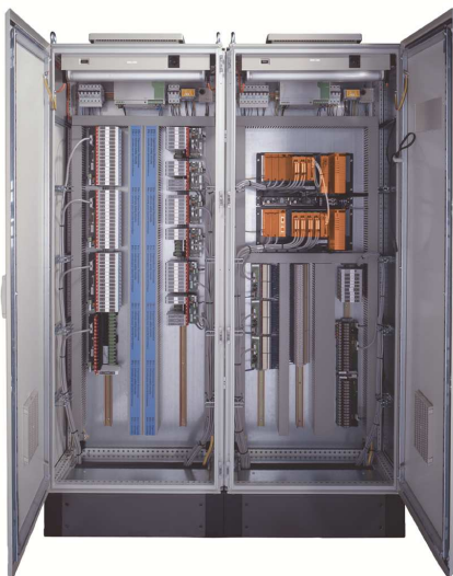
Example of a customer specific field station for a Yokogawa system
